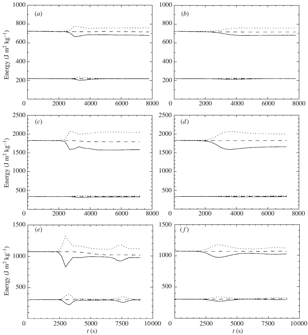
FIGURE 23. Time evolution of kinetic energy (solid curve), potential energy offset by initial kinetic energy (dotted curve), and total energy (dashed curve) for a shoaling wave using narrow shelf with L = 200 m (left column) and wide shelf with L = 600 m (right column). (a, b) Exponential stratification with S = 15 m for initial amplitudes of 7.6 and 14.3 m. (c, d) Mixed-layer stratification for initial amplitudes of 9.6 and 21.2 m. (e, f) Exponential stratification with S = 35 m for initial amplitudes of 6.9 and 14.5 m. (e) L = 200 m. (f) L = 600 m.
