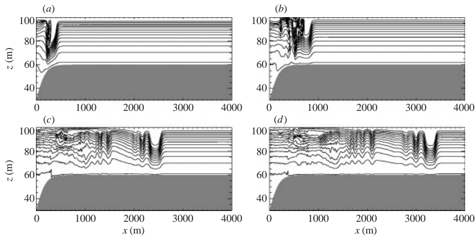
FIGURE 10. Shallowing wave for mixed-layer density. Initial wave amplitude 21.2 m. L = 200 m. (a) t = 50 min, (b) t = 60 min, (c) t = 100 min, (d) t = 120 min.
