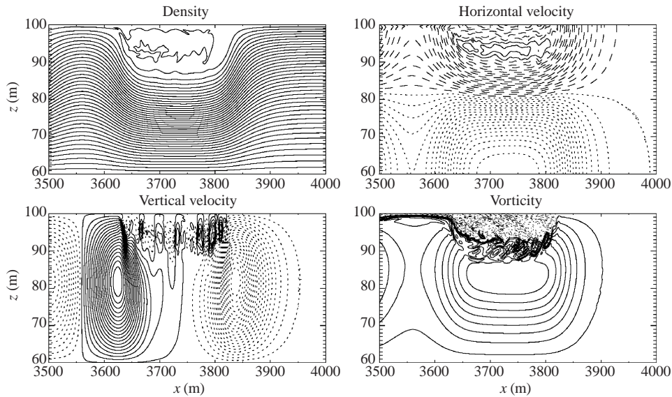
FIGURE 17. As in figure 16 but for wave with trapped core at limiting amplitude. Exponential stratification with S = 35 m, L = 200 m and initial wave amplitude 20.5 m. Solid horizontal vorticity contours are for u > c = 0.59 m s -1 . t = 150 min.
