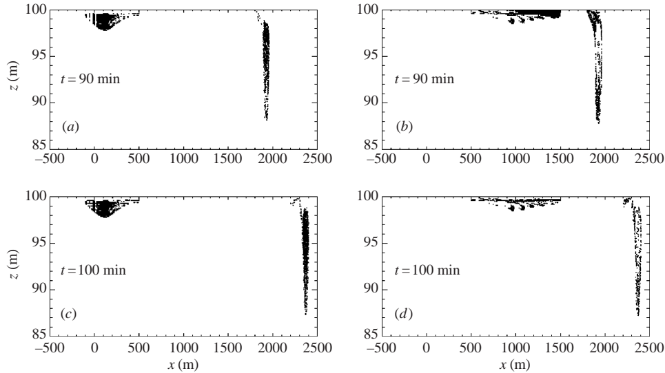
FIGURE 19. Particles in and around the core and their initial locations at t = 90 and t = 100 min. (a, c) Particles with initial horizontal coordinates less than 500 m; (b, d) Particles with initial horizontal coordinates greater than 500 m. Same case as figure 18.
